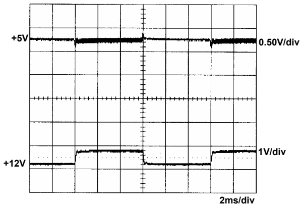
+5V step from 2.3A to 11.5A other output at 60% load
