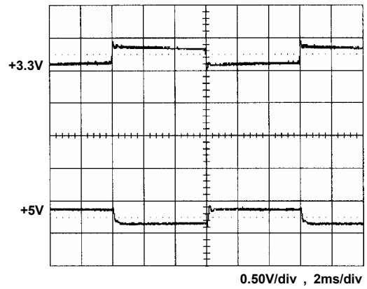
+3.3V step from 2A to 10A other output at 60% load
